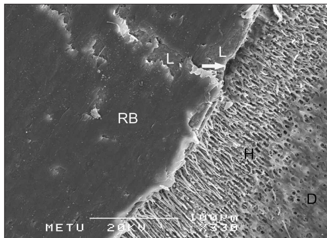
Figure 7: Scanning electron micrographs from the middle section of the interfacial layers between dentin, resin based luting agent and FRD in the RB group. D, dentin; L, luting agent; H, hybrid zone; RT, resin tag; RB, Ribbond (original magnification 330x).
